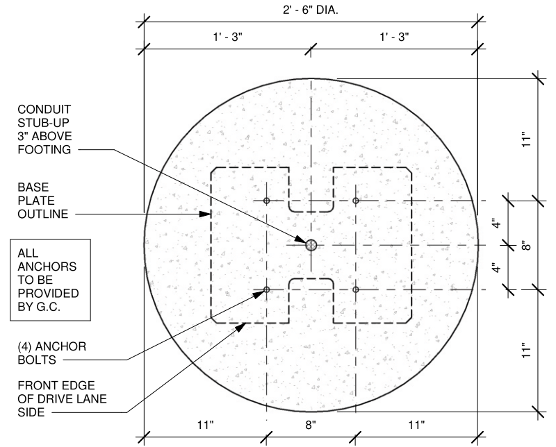
BOLT PATTERN (TOP VIEW) scale: 1" = 1'
