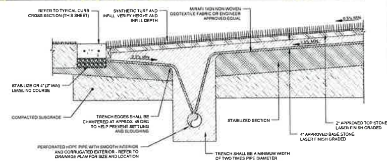
TYPICAL SYNTHETIC TURF CROSS SECTION
