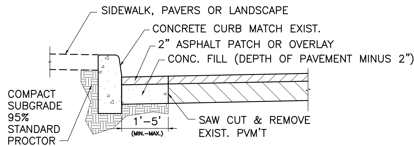
CURB REPLACEMENT
