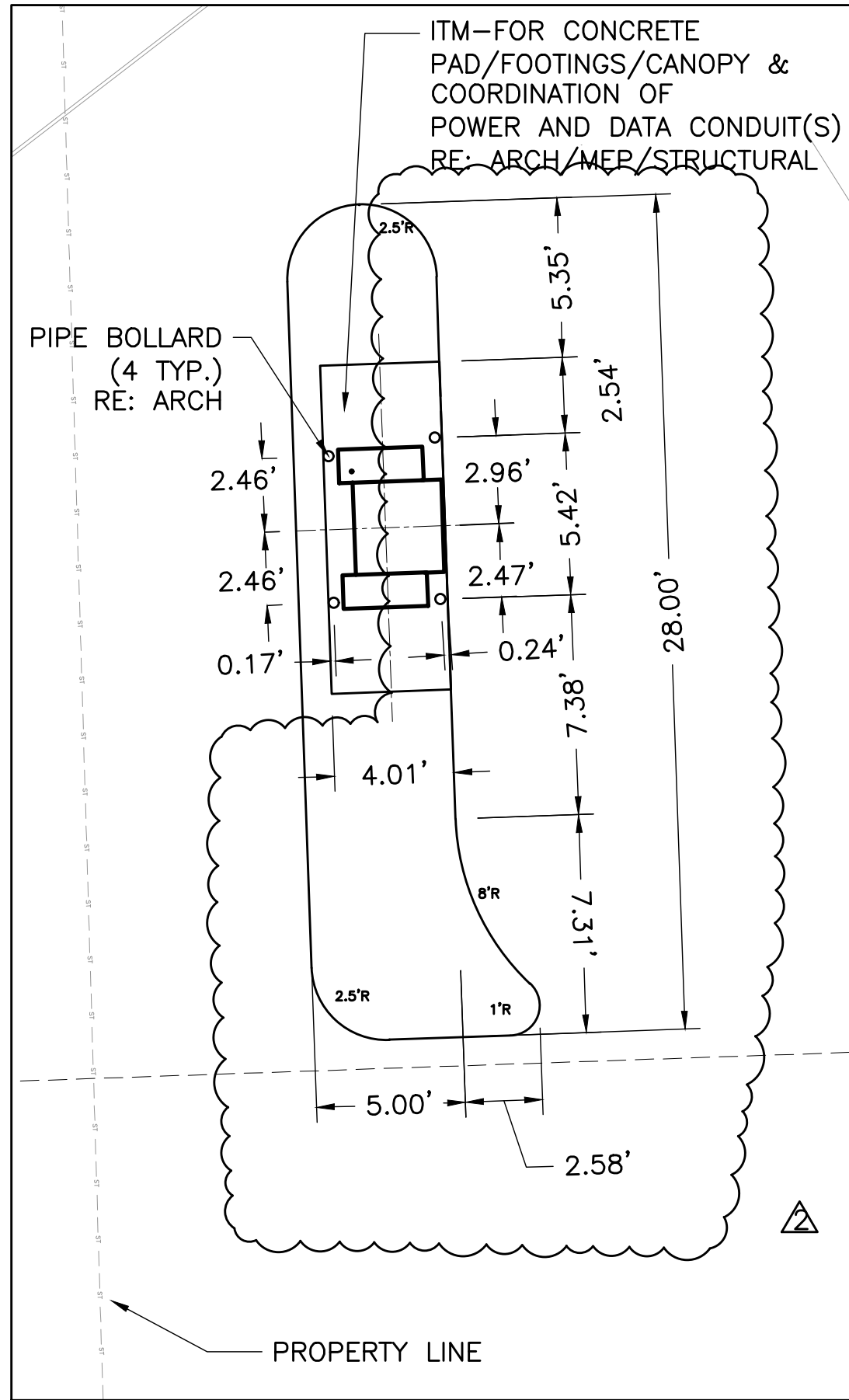
ITM ENLARGED PLAN:
