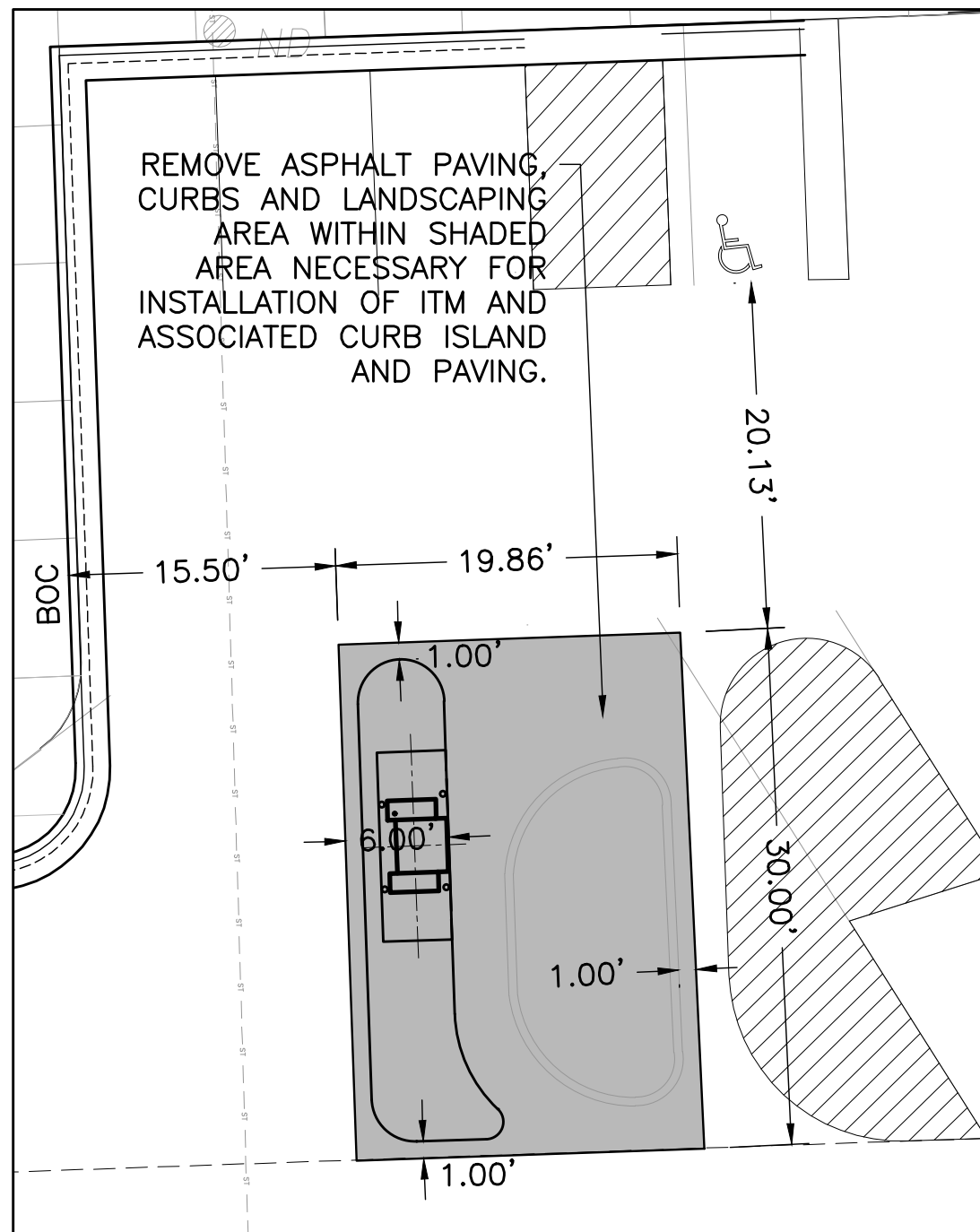
ITM ENLARGED DEMOLITION PLAN:
